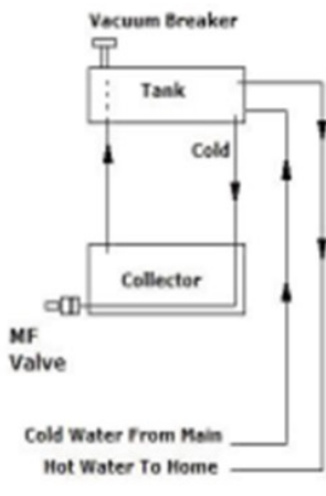
Thermosiphon System
